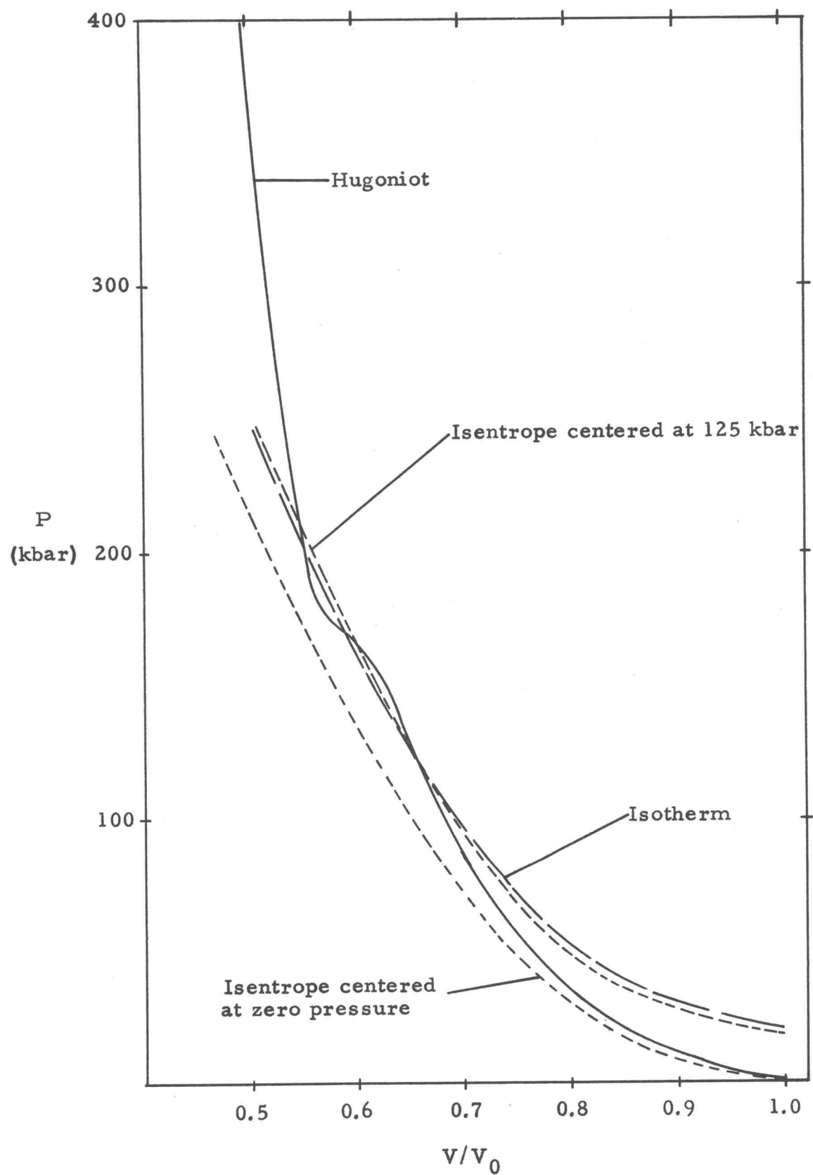
Fig. 25. Benzene isentropes, isotherm, and Hugoniot.
